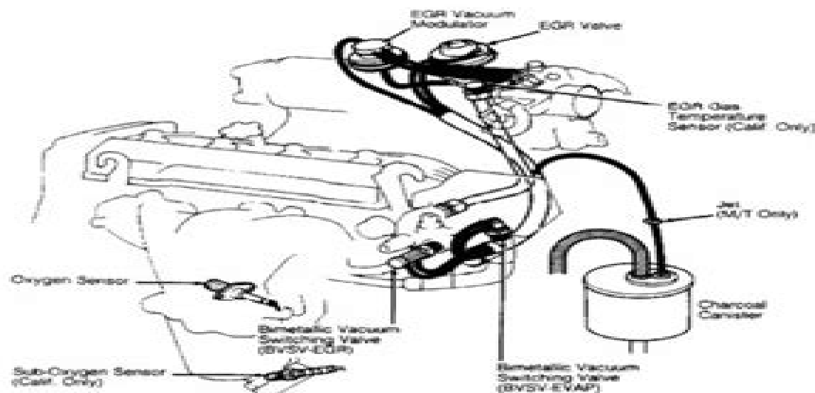
Fig. 1: Vacuum Diagram (Camry 2.0L 1 of 2) Courtesy of Toyota Motor Sales, U.S.A., Inc.
