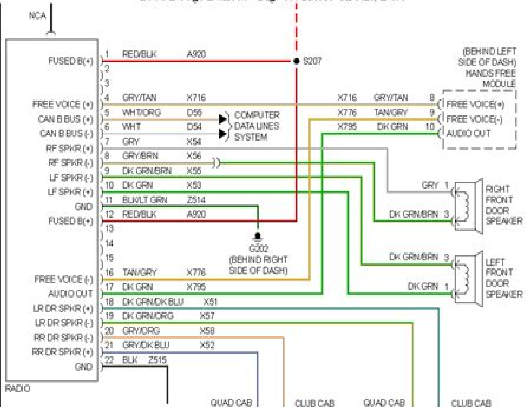
2006 Dodge Dakota - Fig. 40: Radio Circuit, Base
