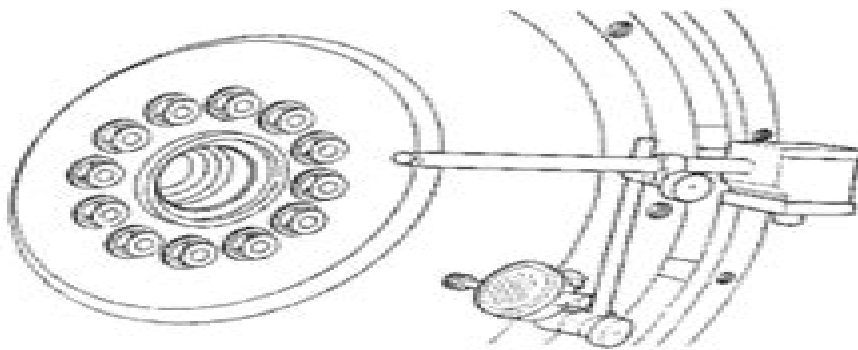
Illustration 2 Face Runout Check
