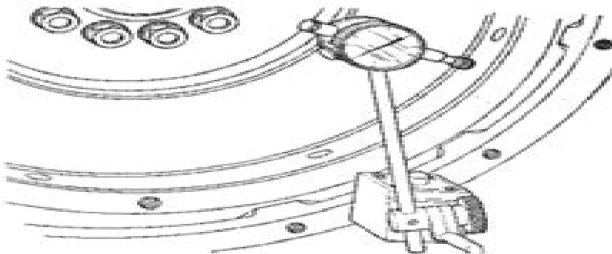
Illustration 3 Bore Runout Check
