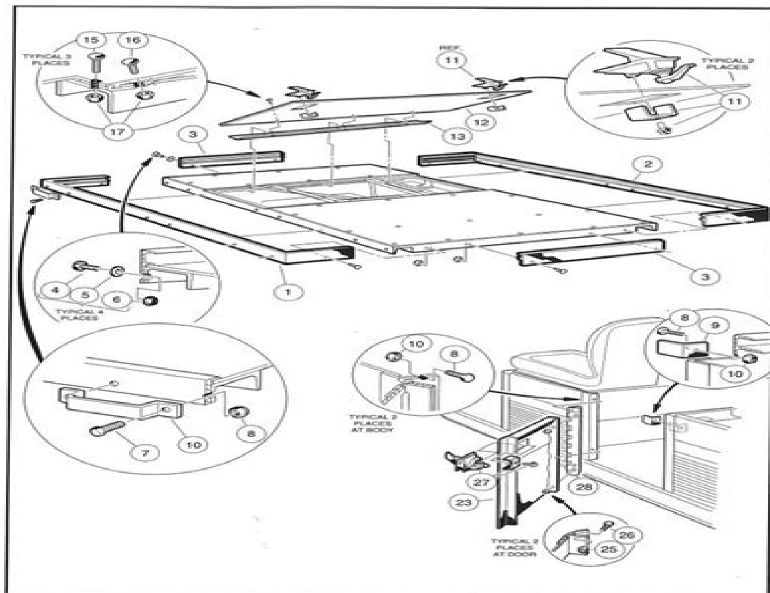
Figure 4-4 Flat Bed Trim, Access Door, and Side Door – Turf 6 and Carryall 6
