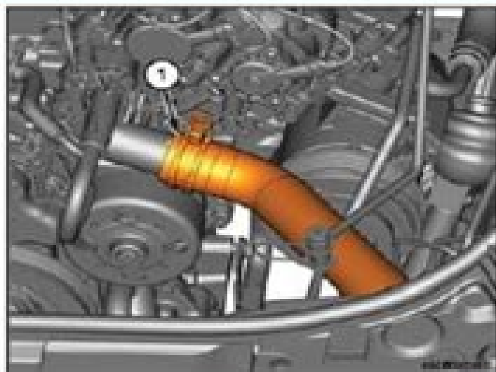
Remove the upper radiator hose (1).
