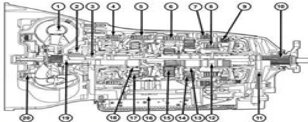
Fig. 1: NAG1 Automatic Transmission Courtesy of CHRYSLER GROUP, LLC
