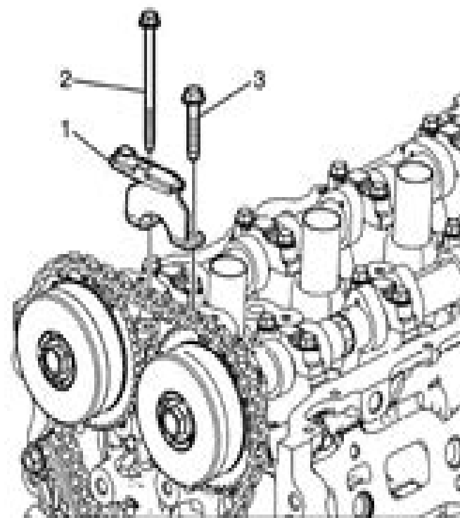
Fig. 242: Upper Timing Chain Guide Bolts Courtesy of GENERAL MOTORS COMPANY
