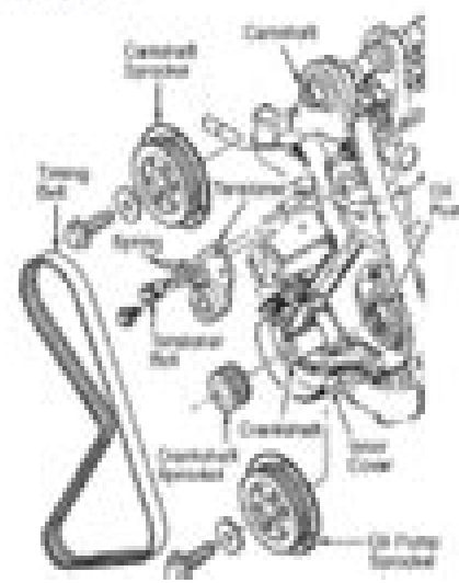
Fig. 5: Aligning Camshaft & Oil Pump Timing Marks Courtesy of Ford Motor Co.
