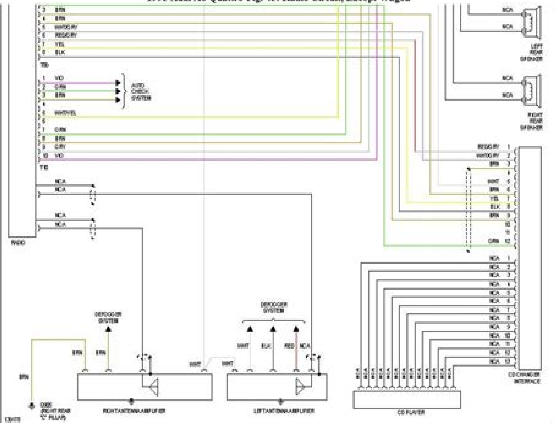
1995 Audi A6 Quattro-Fig. 45: Radio Circuit, Except Wagon
