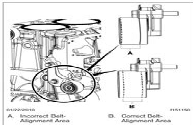
Fig. 3, Idler-Pulley Belt Alignment
