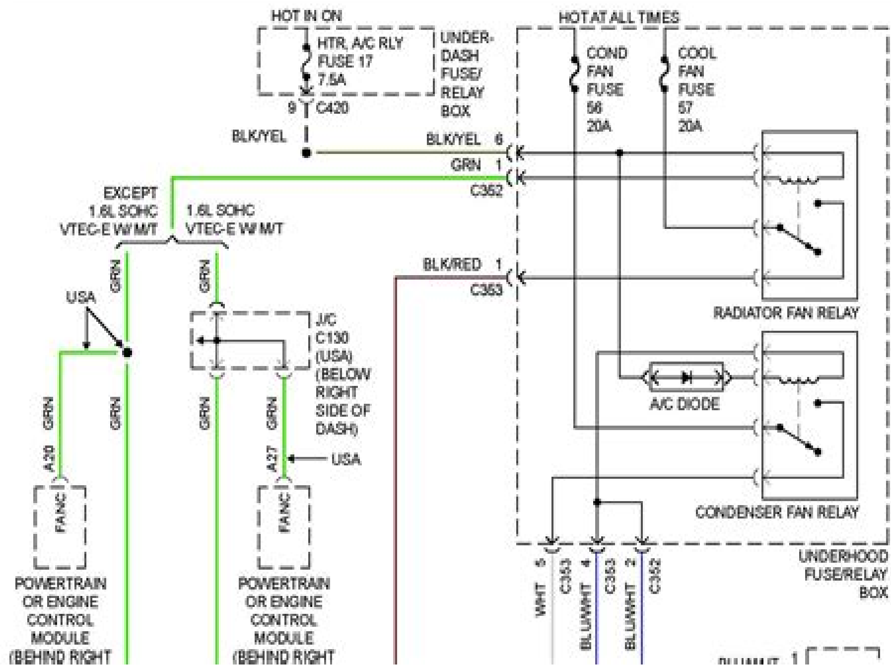
1999 Honda Civic EX- Fig. 9: Cooling Fan Circuit
