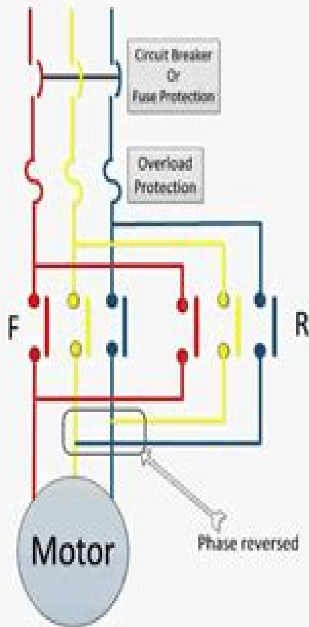
Power Circuit
