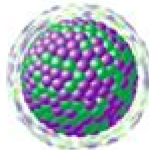
{}_{92}^{236}\text{U} Uranium-236 (very unstable)
