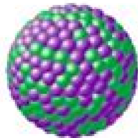
{}_{92}^{235}\text{U} Uranium-235 (fissionable)
