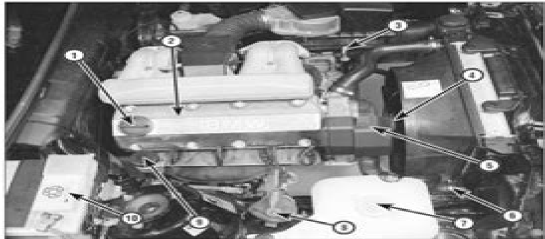
Underbonnet view (right-hand side) of a UK model 318i (1988)
