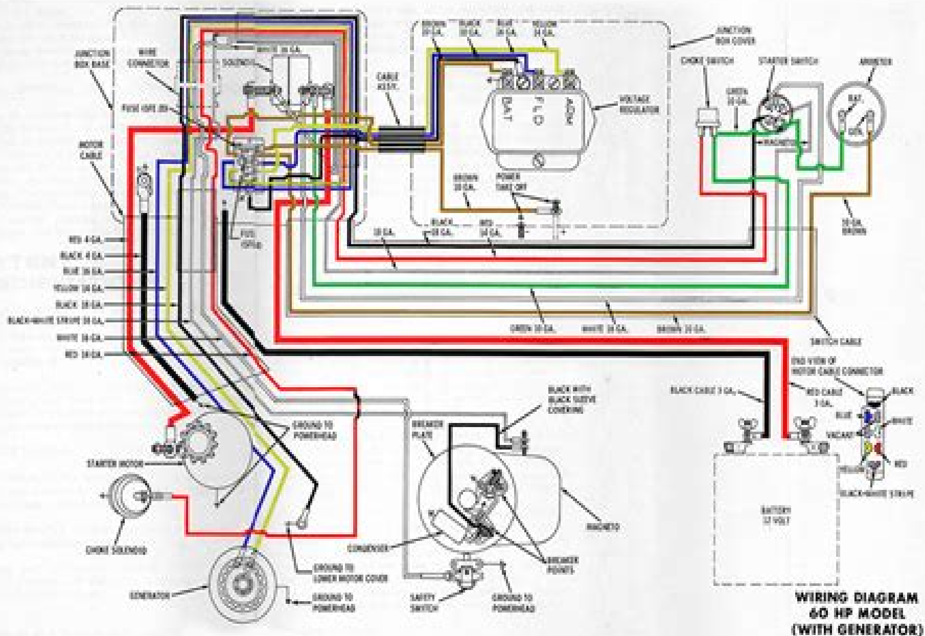
Figure 7-1. Electrical System Schematic
