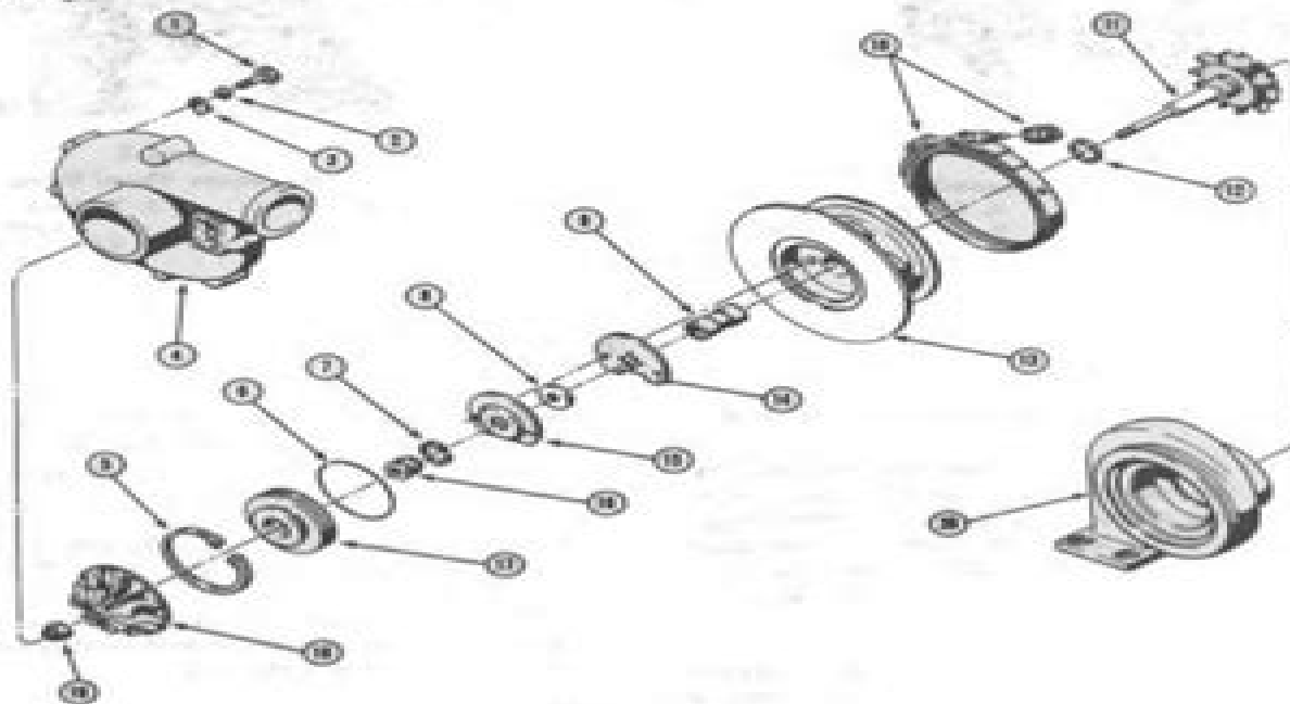
Figure 7 Turboscharger — Exploded View
