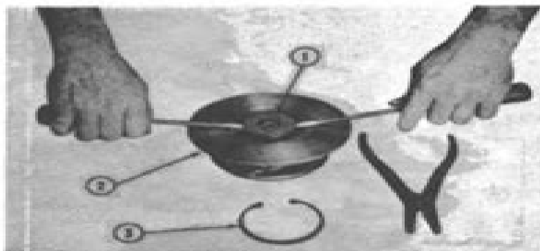
Figure 6 Compressor Insert Removal
