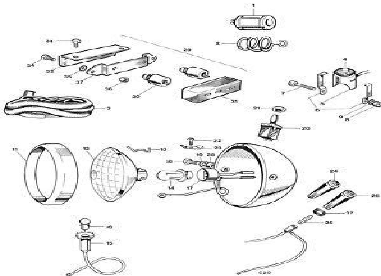
Fig. 31. T190C IGNITION CAPACITOR AND HEADLAMP
