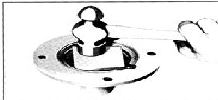
Fig. 7B-23 Installing Main Drive Gear Bearing Retainer Oil Seal
