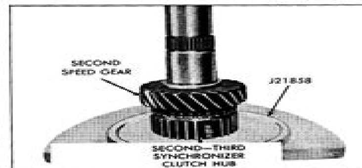
Fig. 7B-24 Installing Second and Third Speed Synchronizer Clutch Hub and Second Speed Gear
