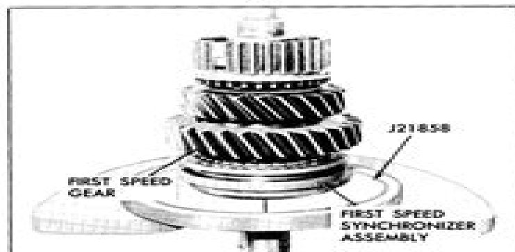
Fig. 7B-25 Installing First Speed Gear and Synchronizer Assembly
