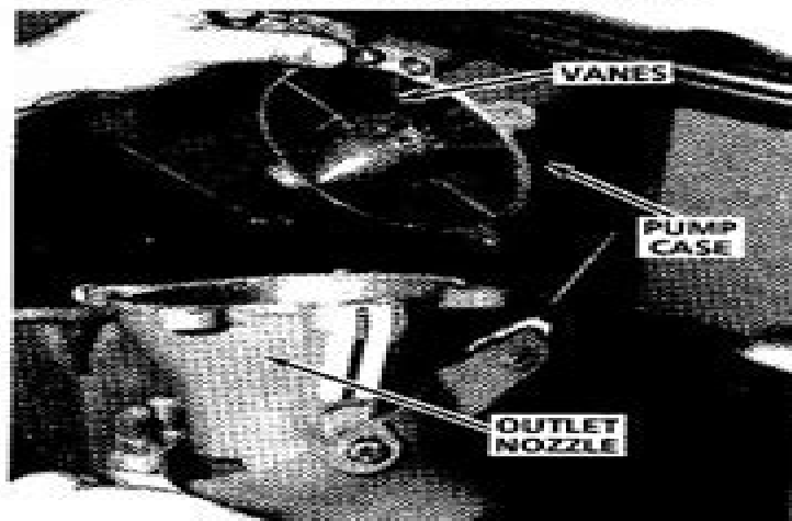
The vanes in the pump case straighten water flow and the conical shape of the outlet nozzle increases flow velocity.
