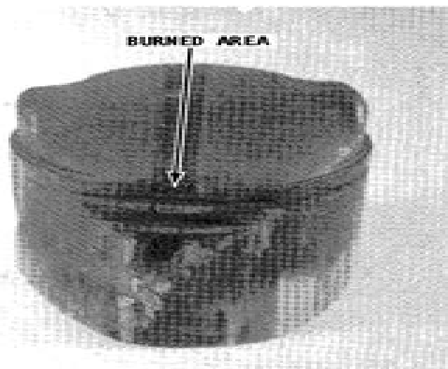
Damaged piston, probably caused by inaccurate fuel mixture, or improper timing.
