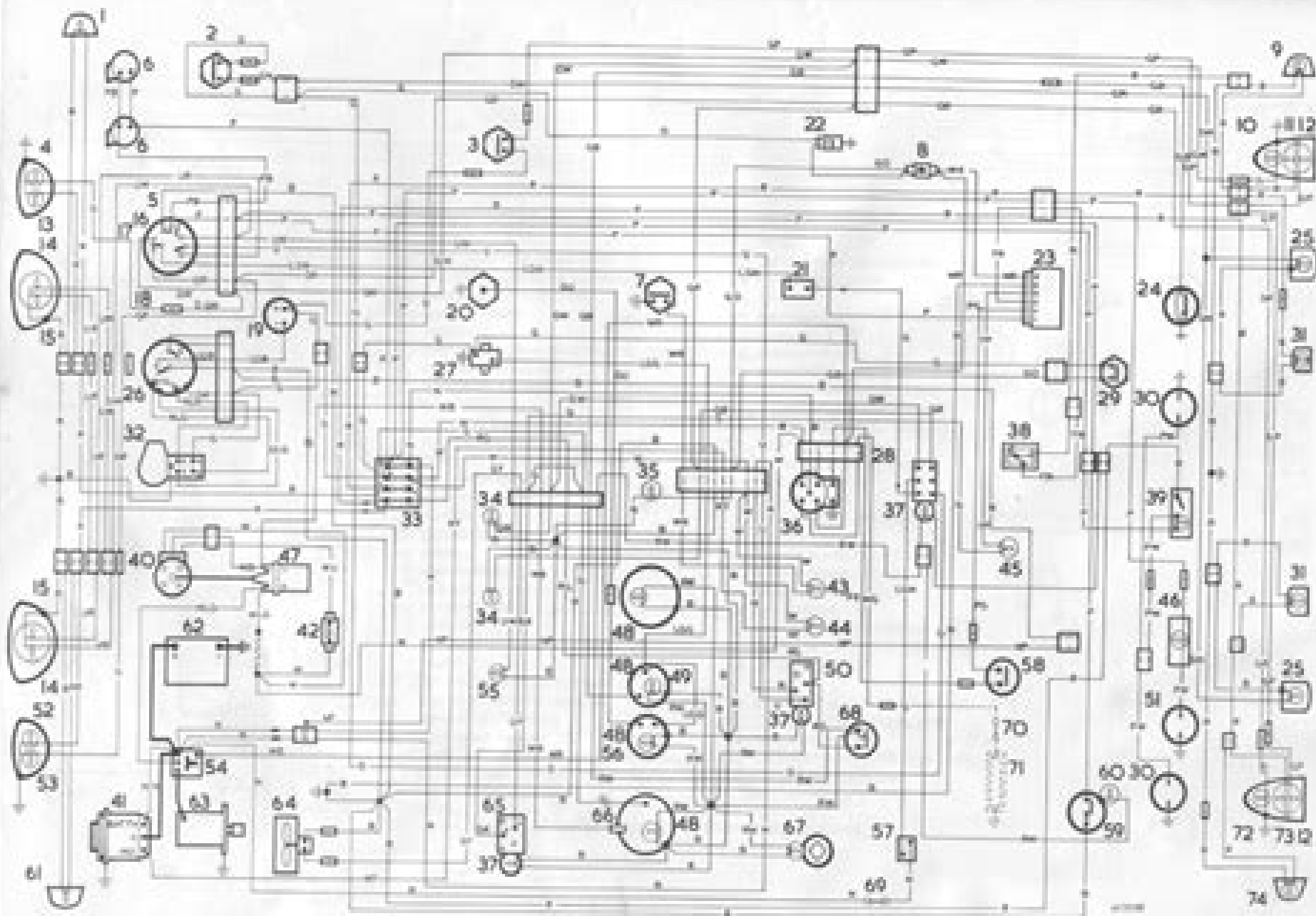
Fig. 10.30 Wiring diagram (USA and Canada, except California) - 1978 onwards
