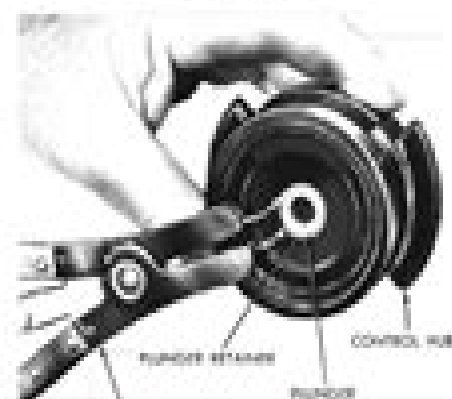
Fig. 11-Removing the Control Hub from the Power Piston Assembly
