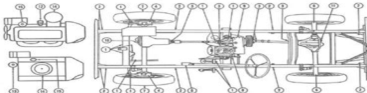
FIG. B-1—LUBRICATION CHART—4-WHEEL DRIVE VEHICLES
