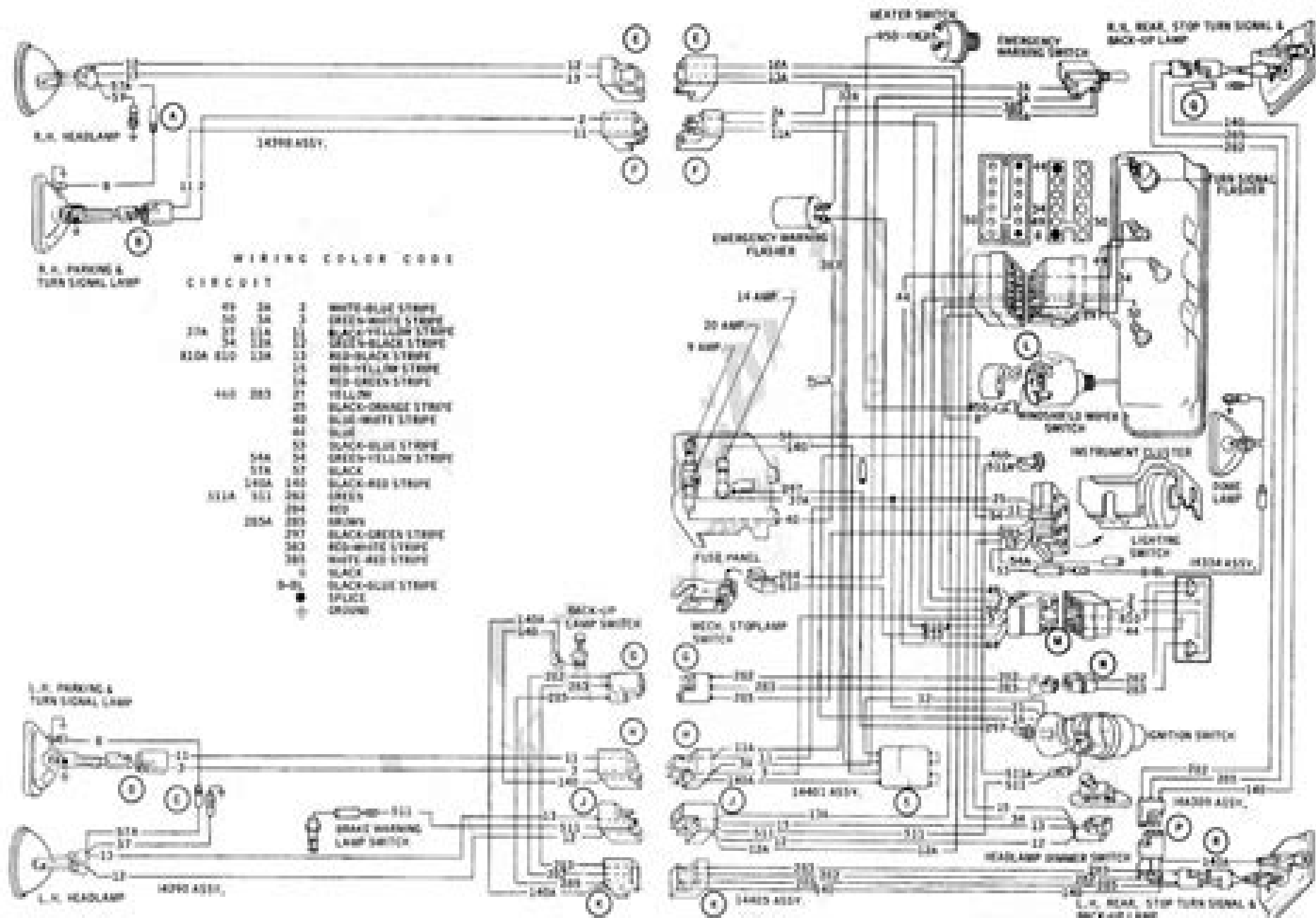
1967 F-100 THRU 350 SERIES TRUCK EXTERIOR LIGHTS AND TURN SIGNALS
