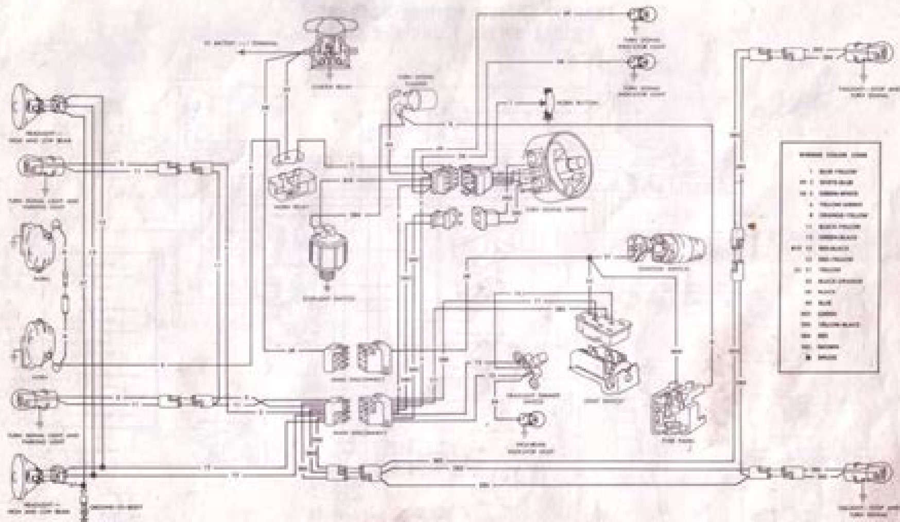
1965 F-100 THRU F-750 SERIES TRUCKS EXTERIOR LIGHTING, TURN SIGNALS AND HORNS
