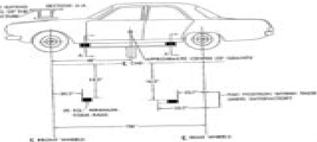
Fig. 2—Support Conditions for Proper Front-Wheel Steering (Steering Wheels)
