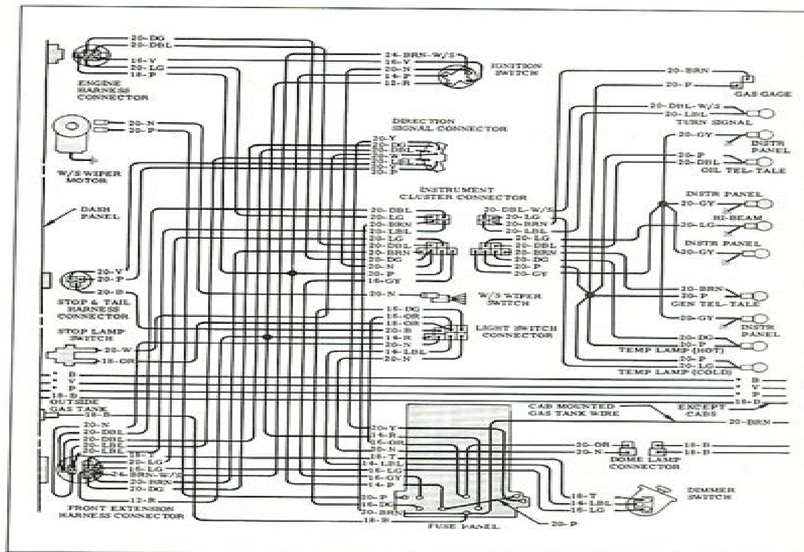
Fig. 43—Instrument Panel and Controls—Models: C-K10-20, C-30 (Except F/P Control)
