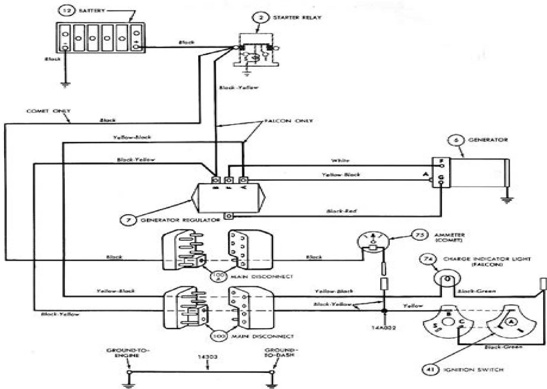
1964 FALCON/COMET GENERATOR SCHEMATIC
