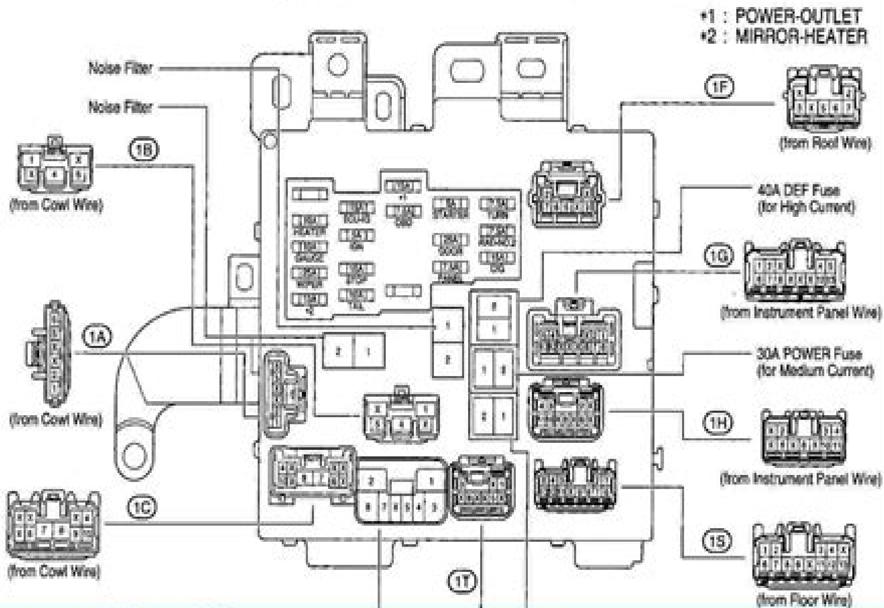
Fig. 2: Identifying Instrument Panel J/B Components Courtesy of TOYOTA MOTOR SALES, U.S.A., INC.
