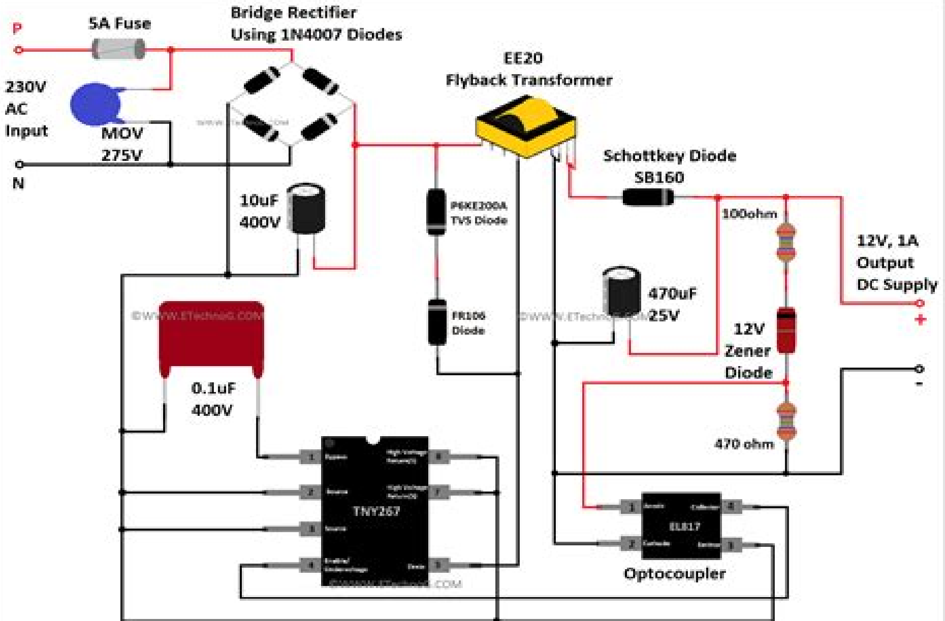
Figure. 01 SMPS Circuit Diagram and Connection(230V/12V)
