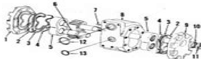
Fig. 8—Exploded view of Plessey hydraulic pump.
