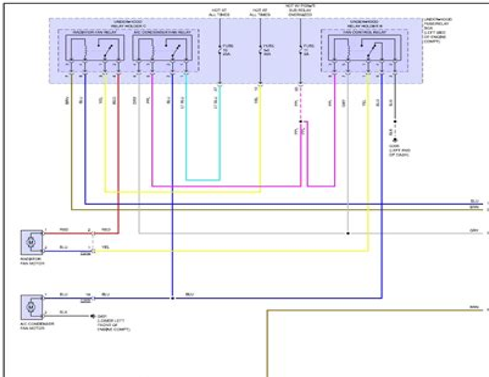
Fig 1: 2.0L Turbo, Cooling Fan Circuit (1 of 2)
