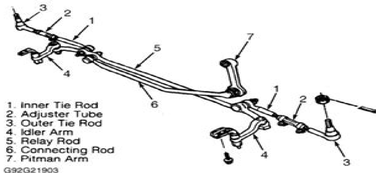
Fig. 3: Exploded View Of Steering Linkage (Astro & Safari - AWD) Courtesy of GENERAL MOTORS CORP.
