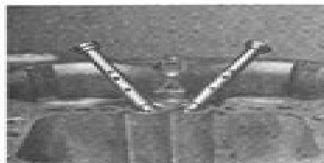
5.13a Removing the emission tubes (DFAV type)
