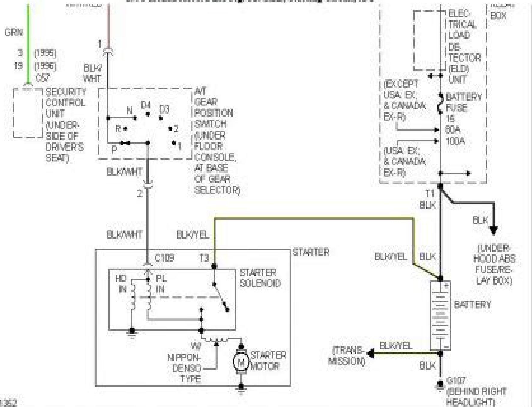
1995 Honda Accord EX Fig. 51: 2.2L, Starting Circuit, AT
