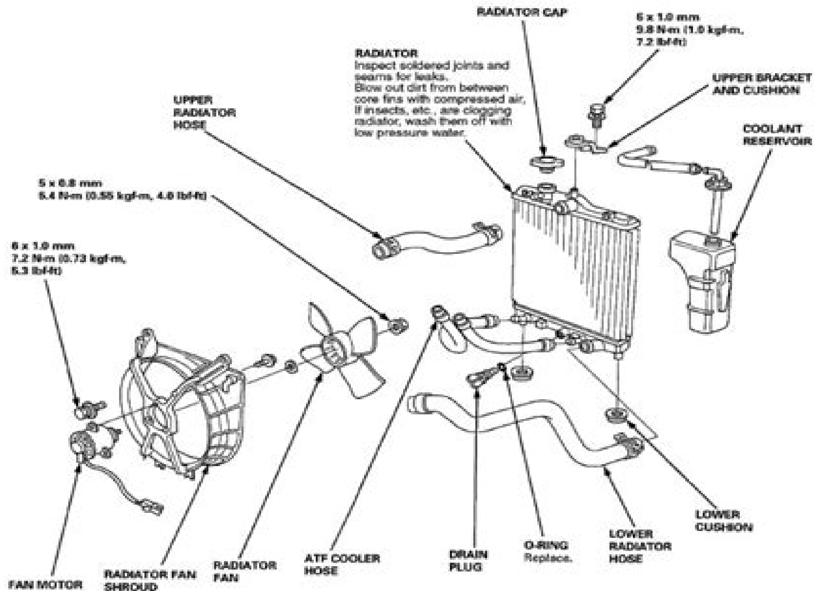
Fig. 1: Exploded View Of Engine Cooling Components AMERICAN HONDA MOTOR CO., INC.
