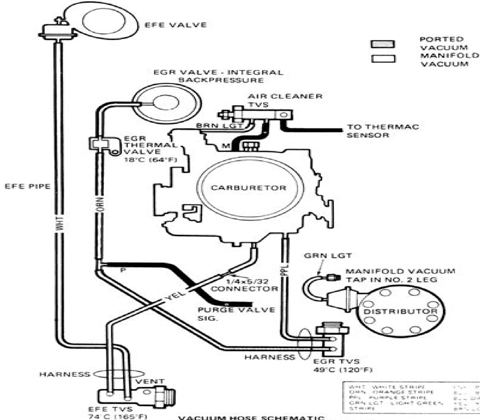
VACUUM HOSE SCHEMATIC (EMISSION SYSTEMS EXCEPT EVAP CANISTER)
