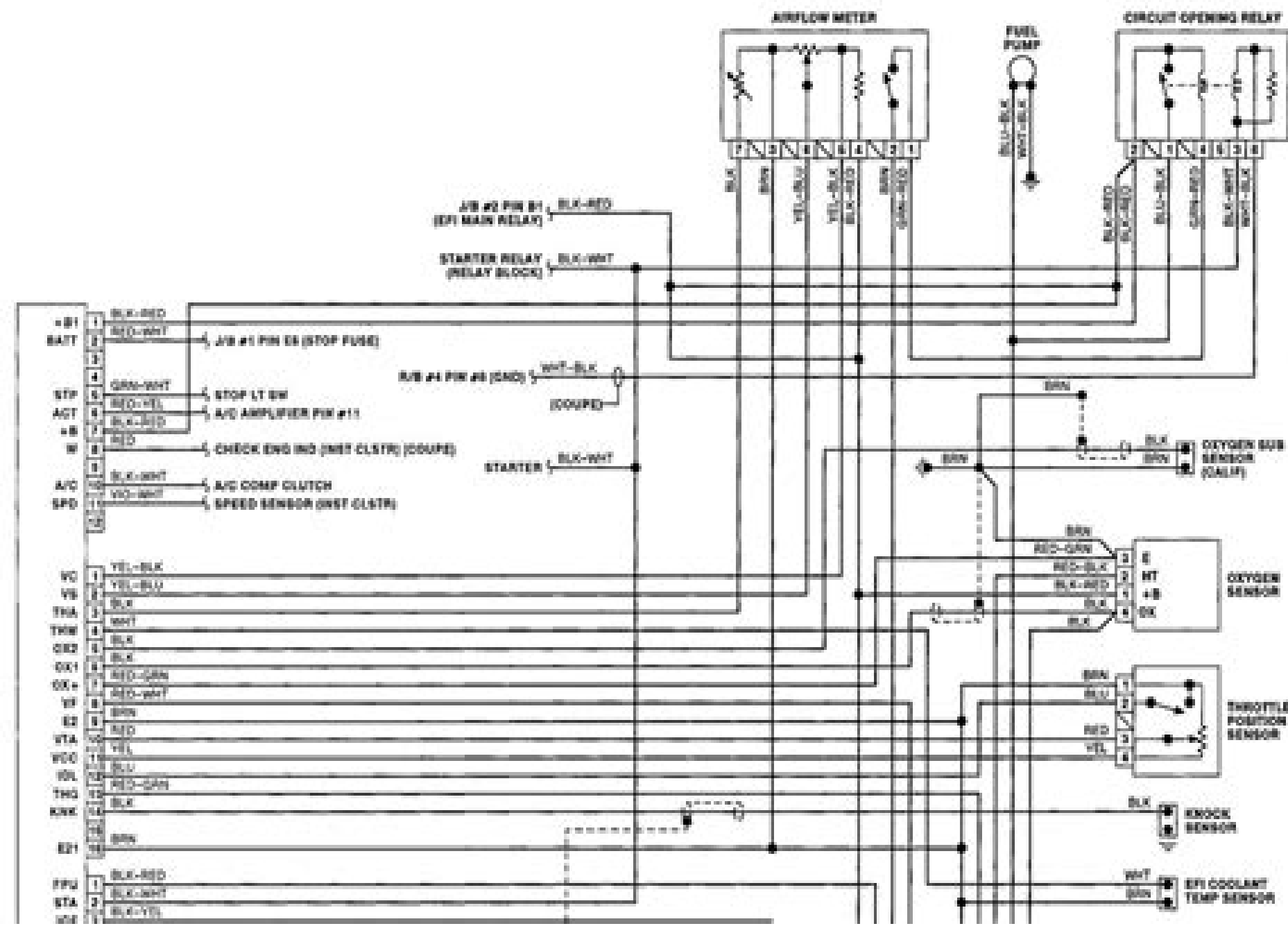
Fig. 3: Computer Engine Control (1.6L 4A-GE) (Grid 8-11)
