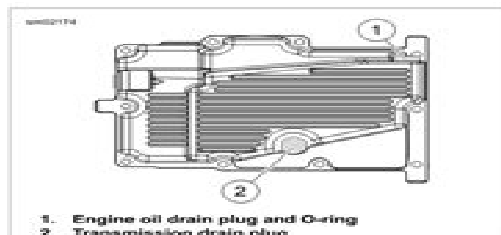
Figure 1-19. Oil Pan
