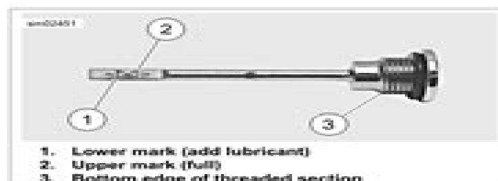
Figure 1-18. Filler Plug/Dipstick
