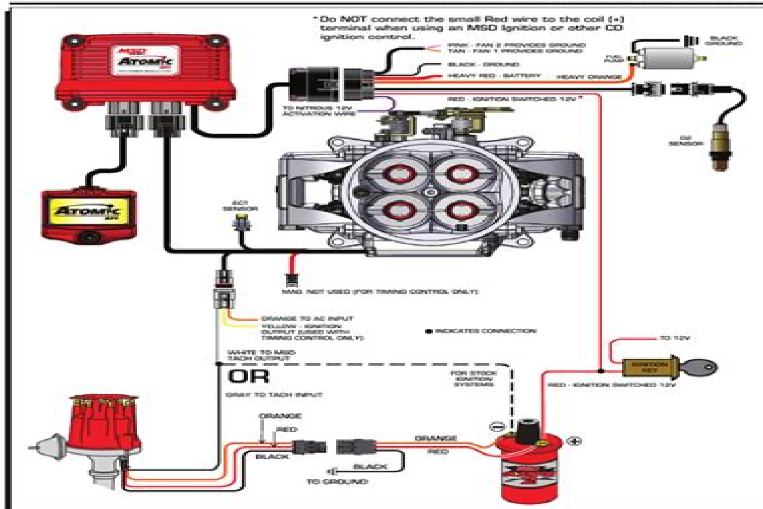
Figure 9 – Atomic Wiring with an MSD Ready-to-Run Distributor or MSD HEI Distributor.
