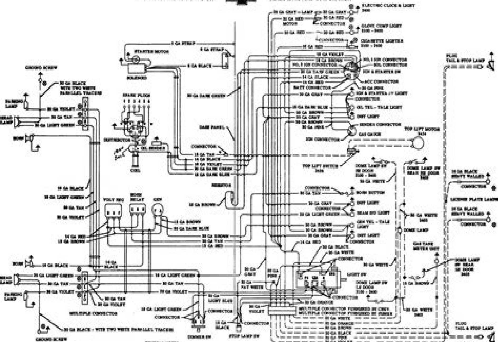
WIRING DIAGRAM
