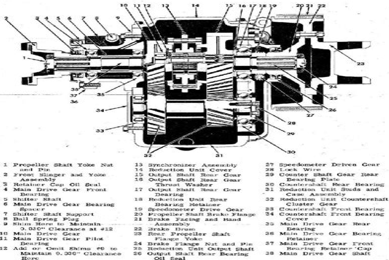
Figure 162—Two-Speed Reduction Unit (Series M350-24 Through M470-30 Only)
