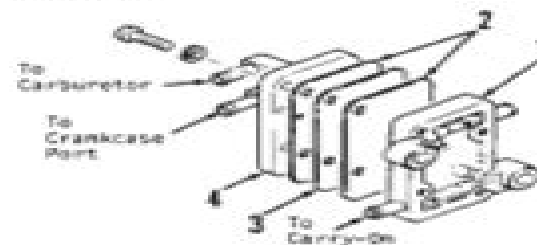
Fig. S24-3—Exploded view of diaphragm type fuel pump.
