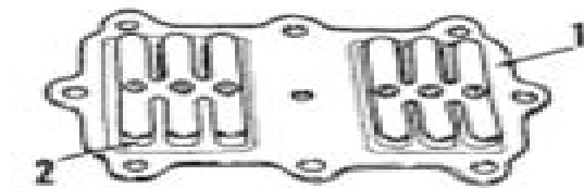
Fig. S24-5—View showing reed plate (1) and reed valve (2) assembly used on DT6 and DT8 models.
