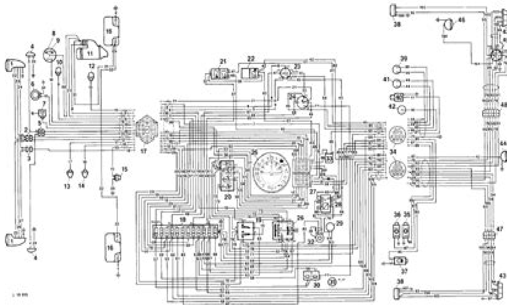
Fig. 1 — Wiring Diagram ("Blue" System), Tractors without Operator's Cab
