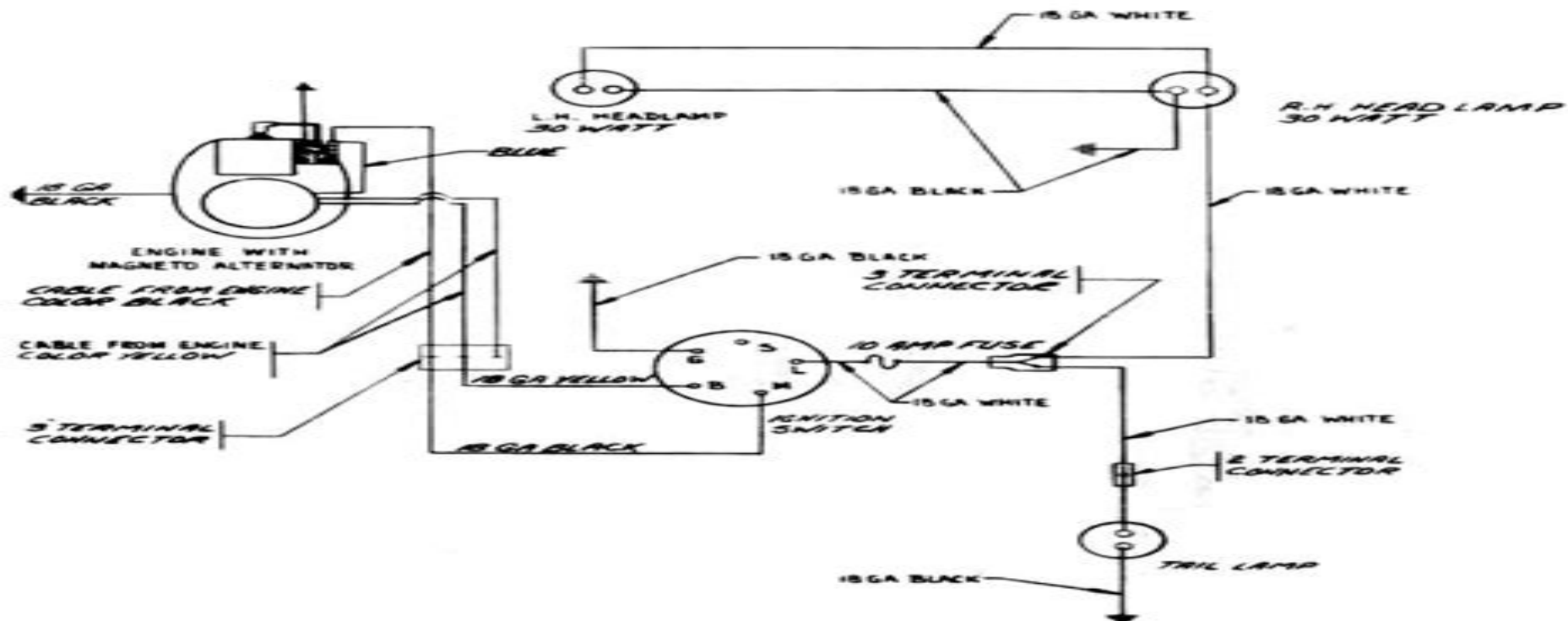
Fig. 25 - Schematic - Manual Start Wiring - Models 300 S, 350 SS
