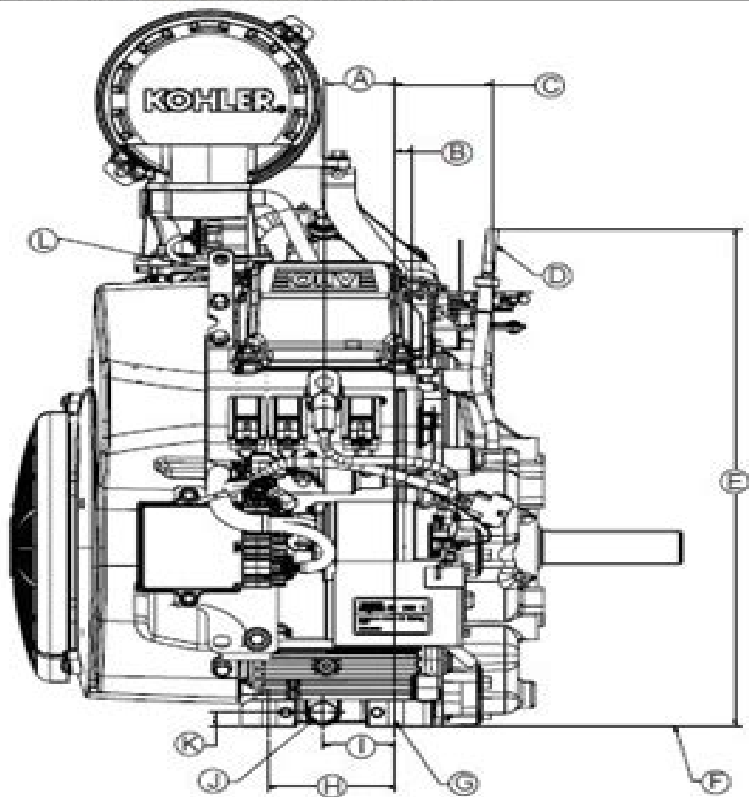
Engine Dimensions with Heavy-Duty Air Cleaner- Starter Side
