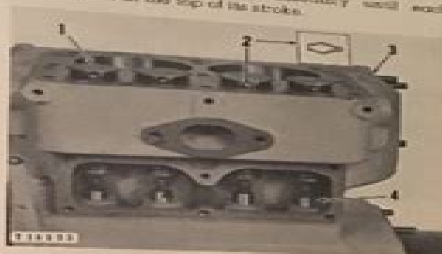
CAMSHAFT REMOVAL SEPARATELY 1-Valve, 2-Large cotter pin, 3-Cylinder block, 4-Lifter assembly.
