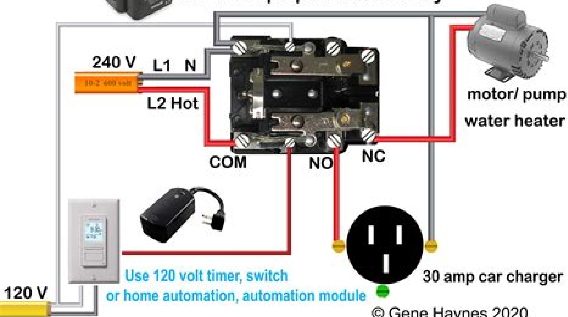
30-40 Amp open-frame relay
