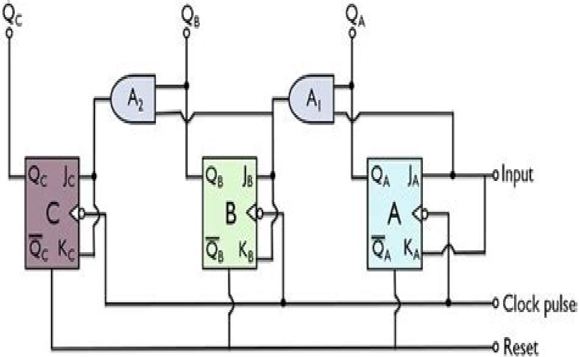
Circuit Diagram of 3-bit Synchronous Counter
