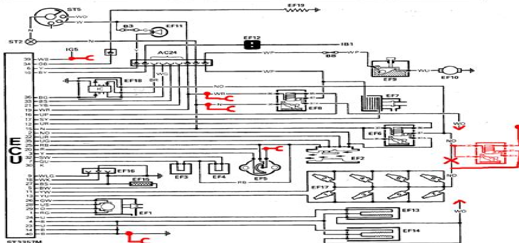
Hot Wire EFI - Circuit Diagram
